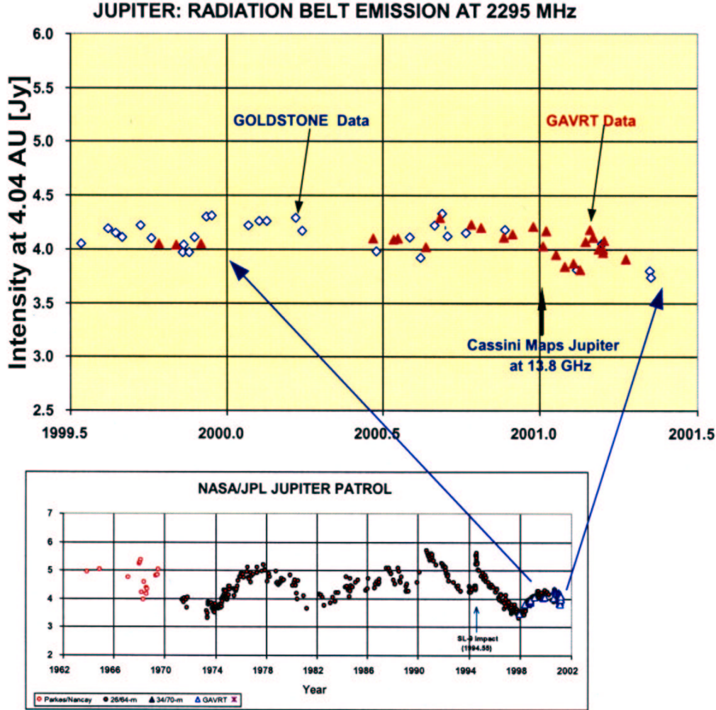
Figure 1: Variations in the intensity of the microwave radio emission from Jupiter's radiation belts.
