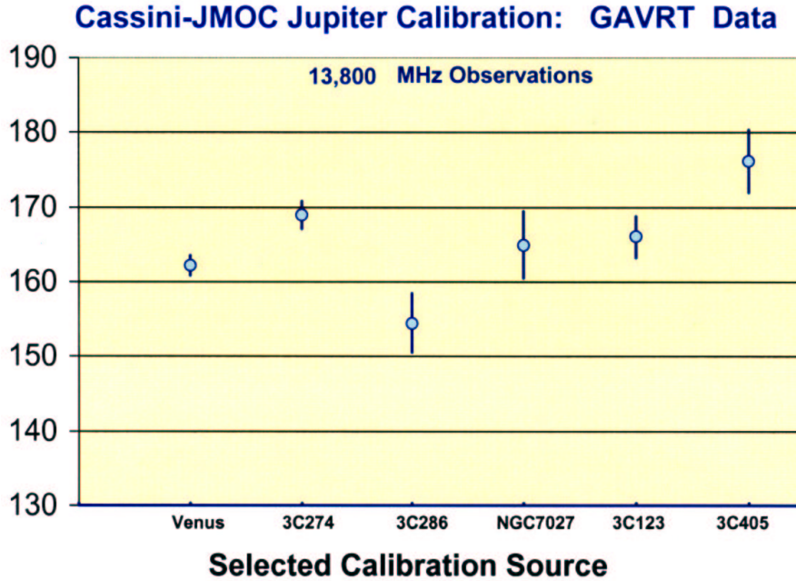
Figure 2: The values of Jupiter's disk temperature at 13.8 GHz derived from the observed ratios of Jupiter relative to six different calibration radio sources.
